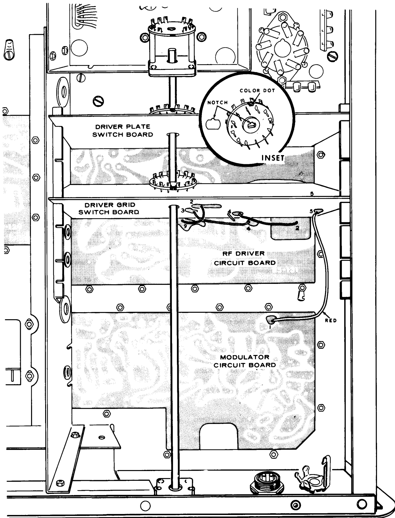
PICTORIAL 8-17
