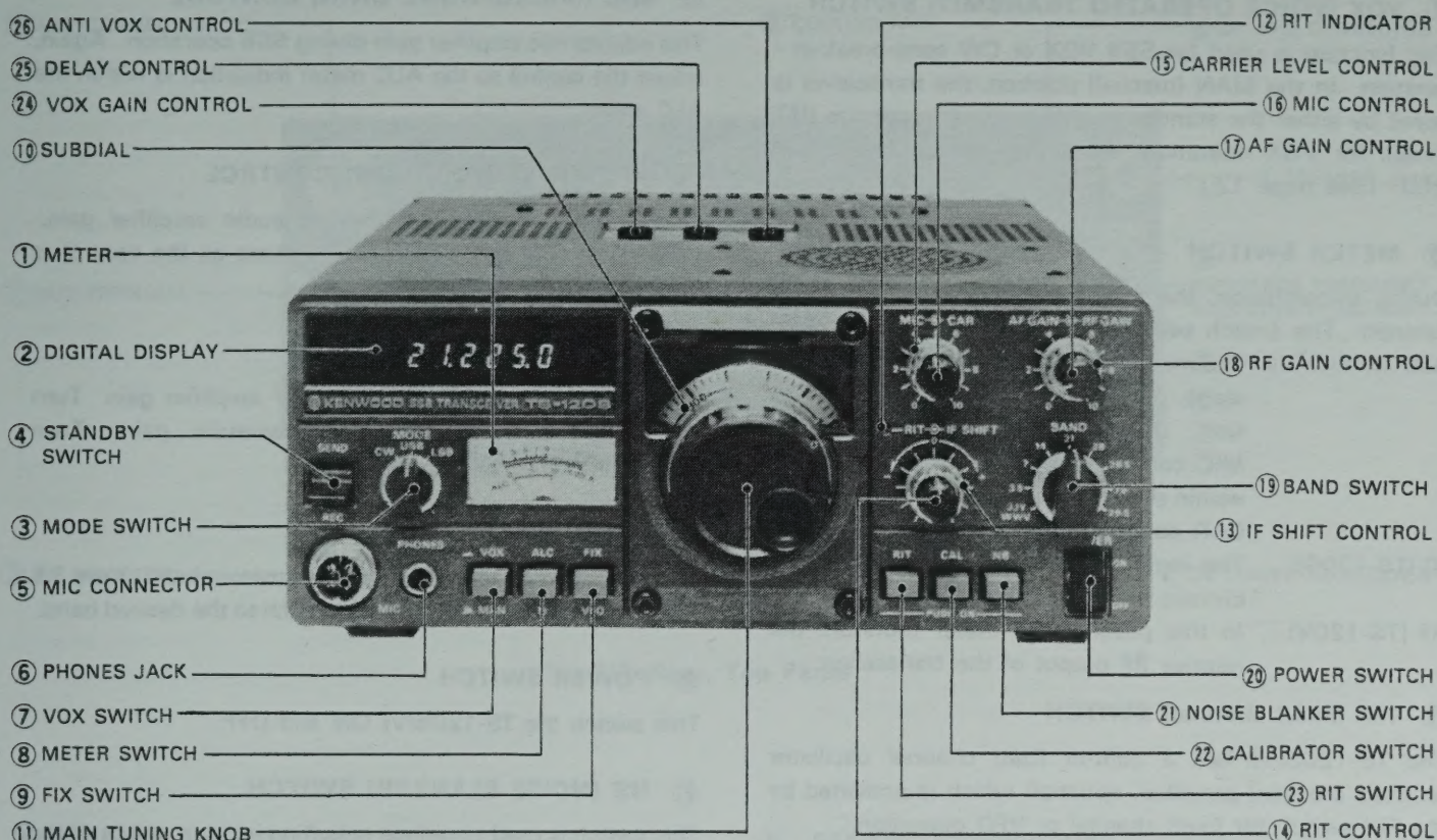
Fig. 3-1 Front Panel
