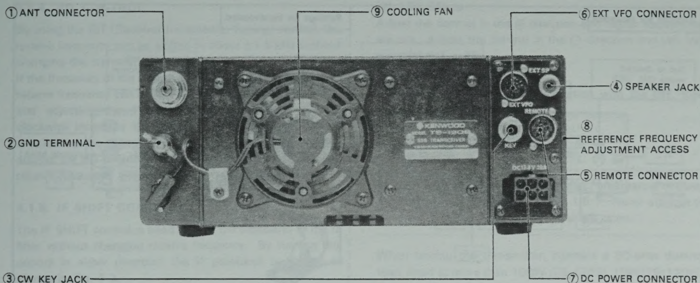
Fig 3-2 Rear, Top Panel
