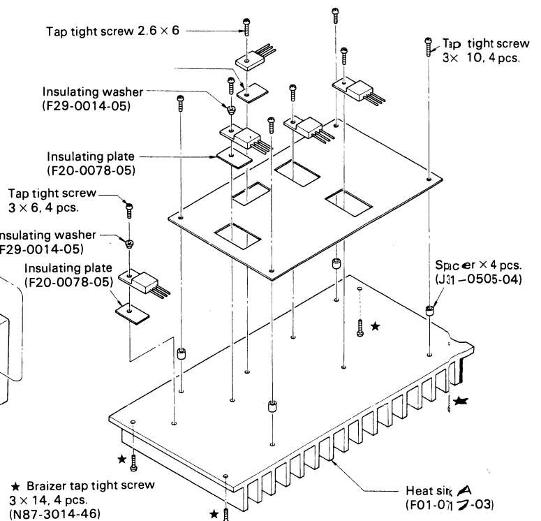
Fig. 13 Final unit disassembly
