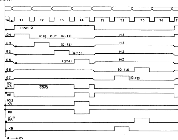
Fig. 4 Timing chart
