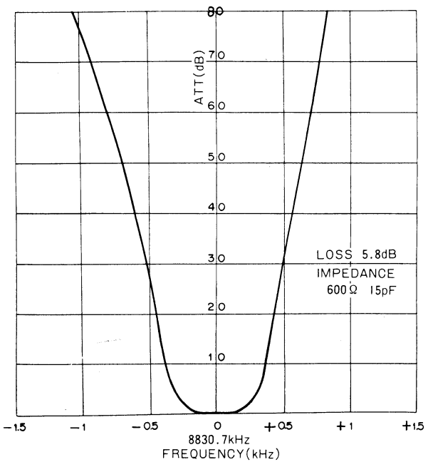
Fig. 20 YK-88C filter attenuation characteristic
