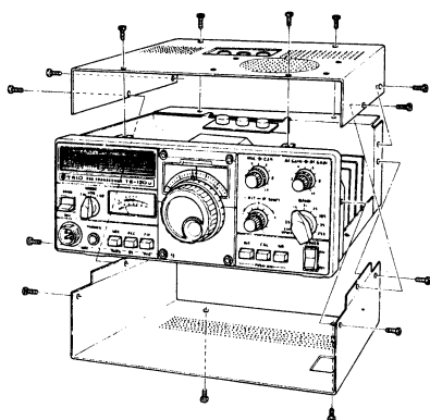
Fig. 14 Case disassembly
