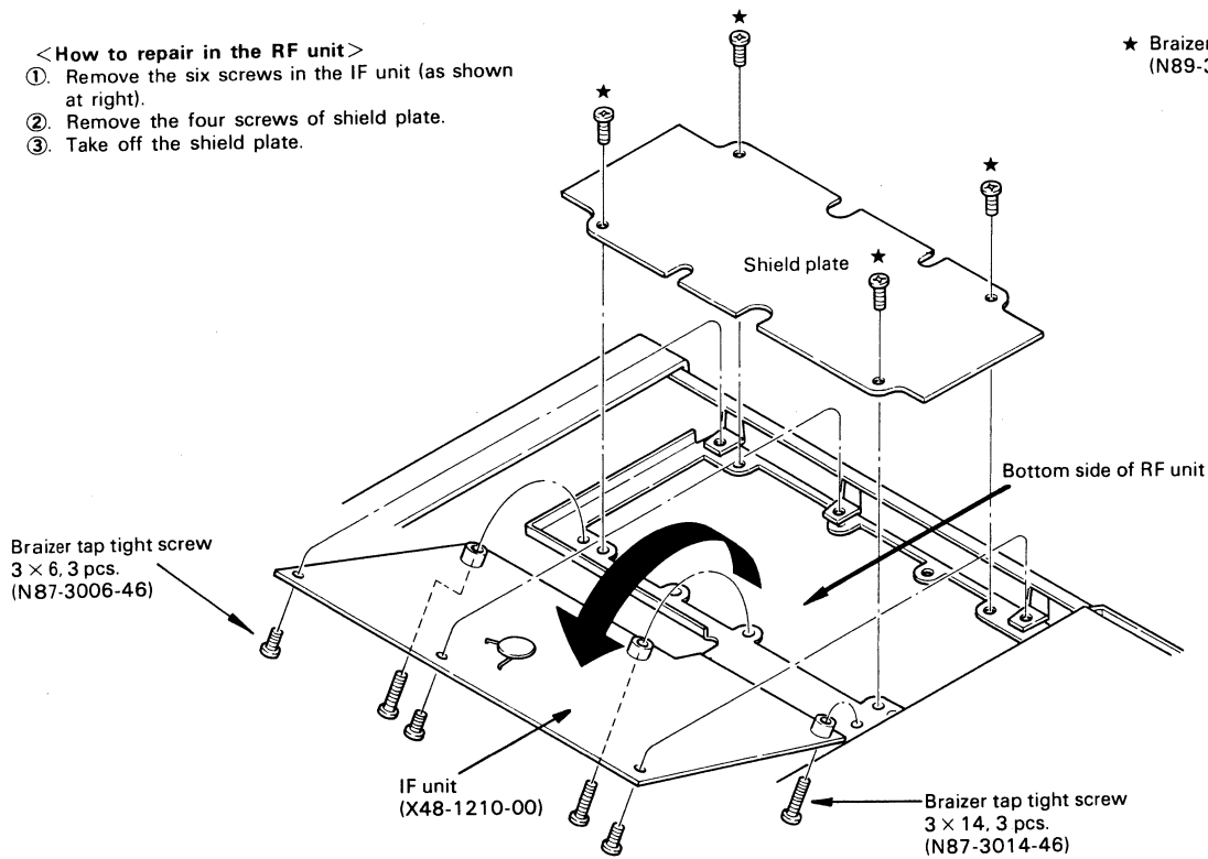
Fig. 11 Repairing the RF unit
