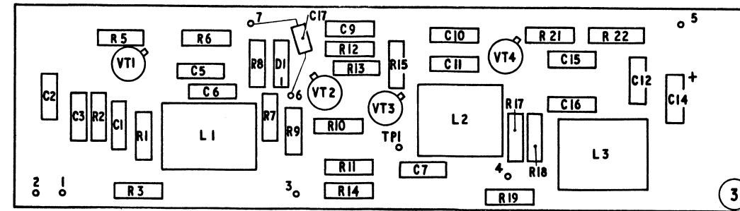
MAIN I.F. AMPLIFIER BOARD
