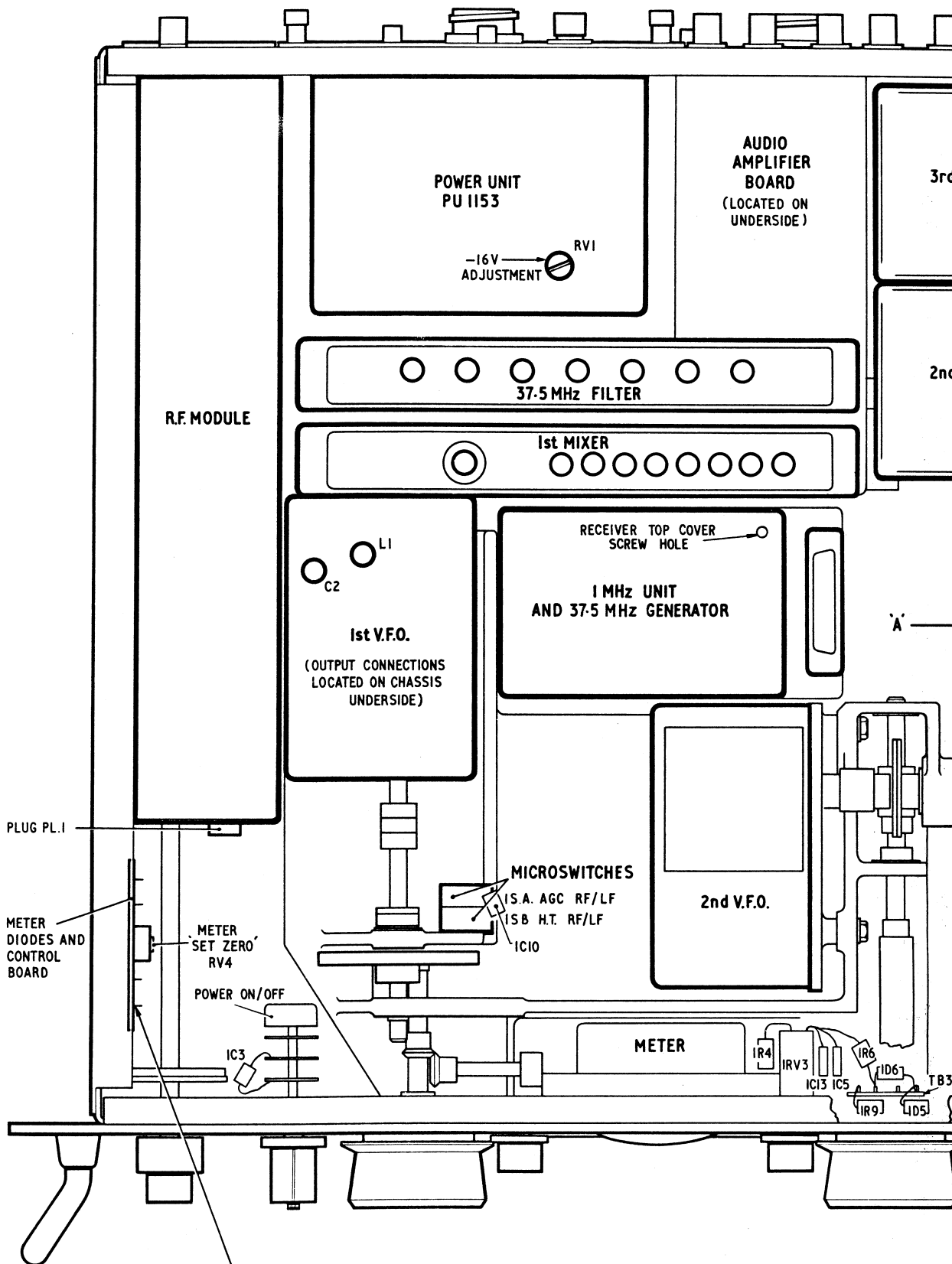
RECEIVER CHASSIS (UPPERSIDE)
