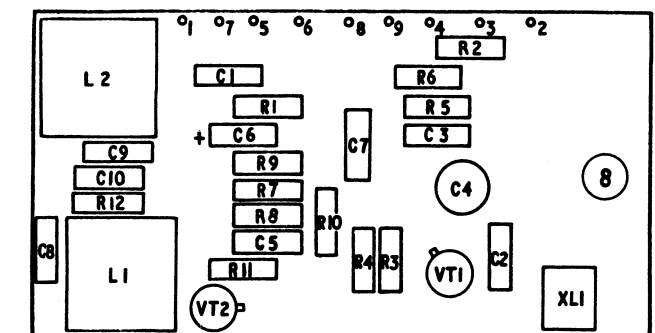
CONVERTER: OSCILLATOR AND MIXER
