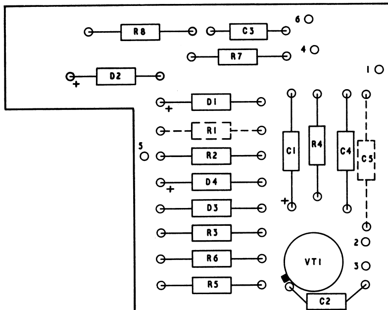
OSCILLATOR BOARD (BA.35808)
