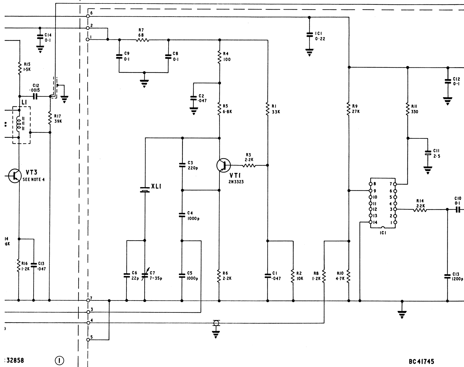
Circuit : 1MHz Amplifiers,Oscillator and Calibrator
