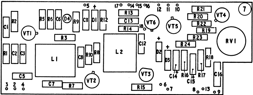
A.G.C. BOARD
