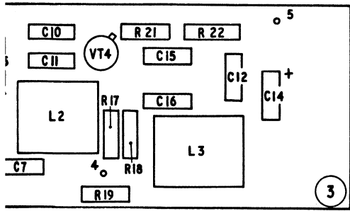
AMPLIFIER BOARD
