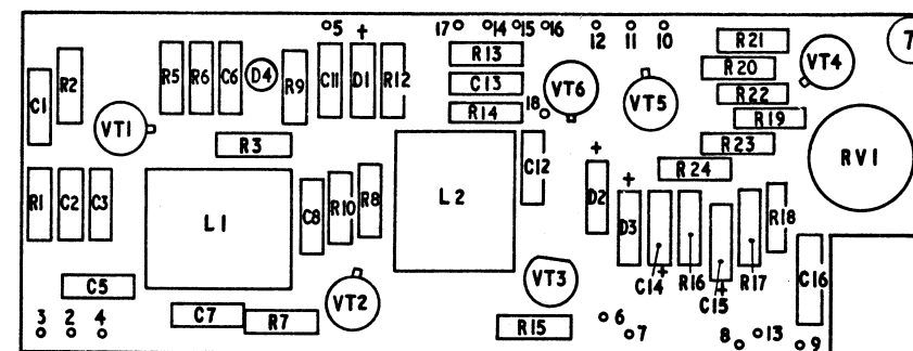
A.G.C. BOARD
