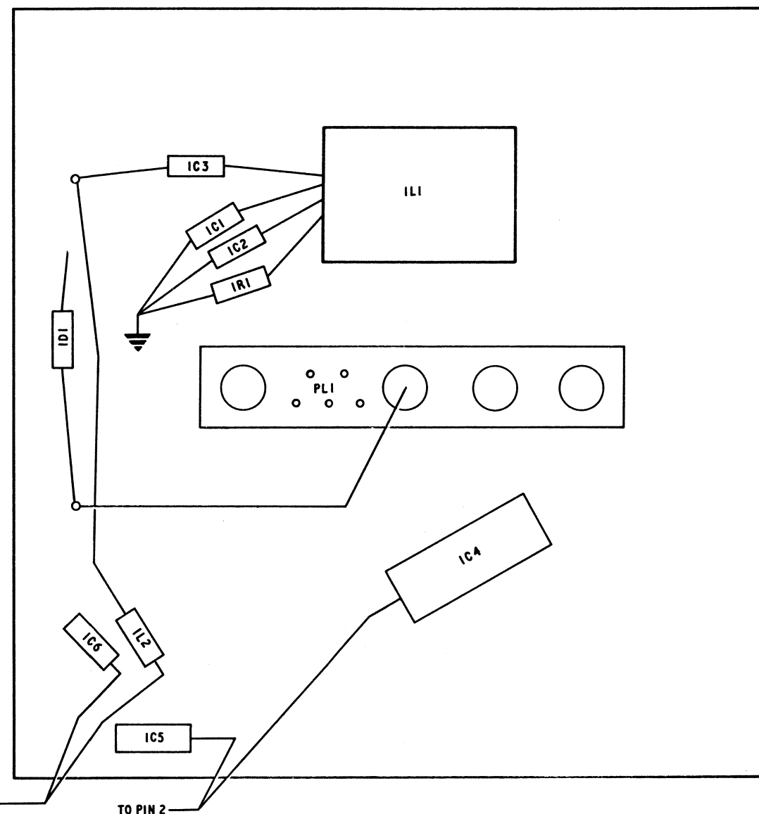
3rd MIXER MODULE (BA 35966)
