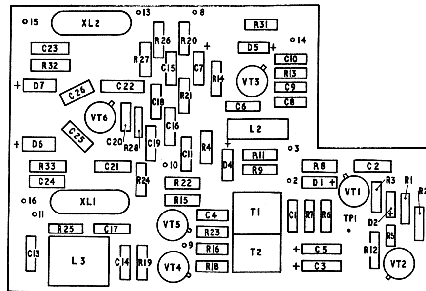
DETECTOR BOARD
