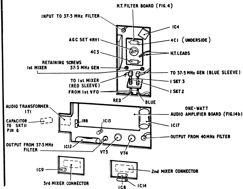
RECEIVER CHASSIS (UNDERSIDE) (WITH ONE-WATT AMPLIFIER)
