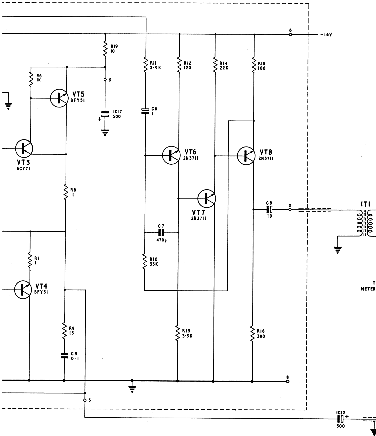
Circuit: Audio Amplifier Board (1 Watt)
