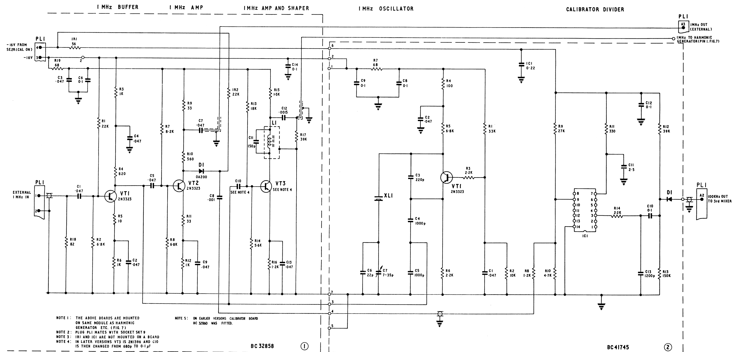
Circuit : 1MHz Amplifiers,Oscillator and Calibrator
