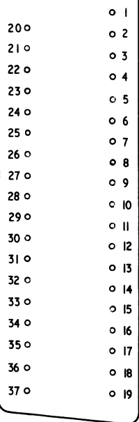
37-WAY CONNECTOR TYPE DCM37S PIN IDENTIFICATION
